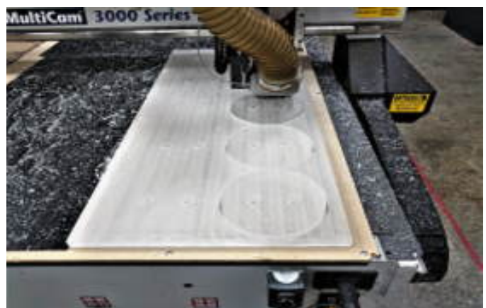
One of our 5' x 10' CNC routers in action.
