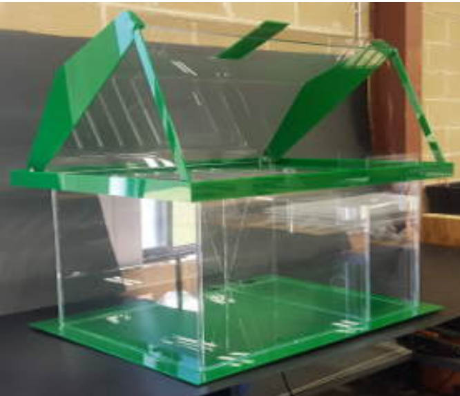
Water tight acrylic bath for Laboratory testing of parts.
